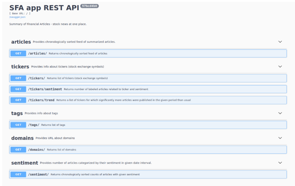
Fig. 2: Auto-generated documentation
