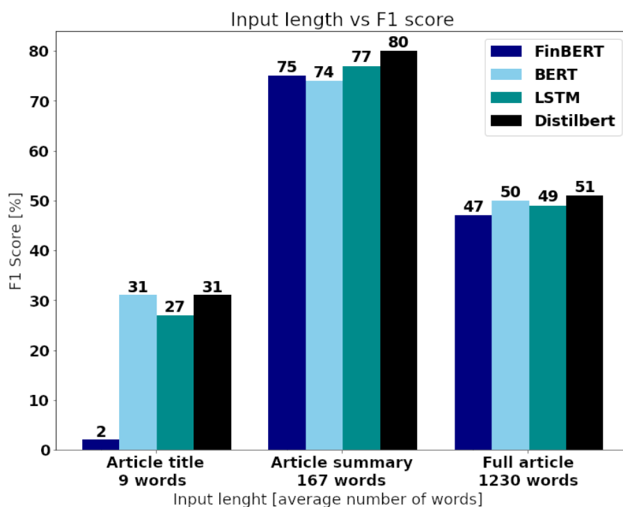
Fig. 4: Performance of methods depending on input length
