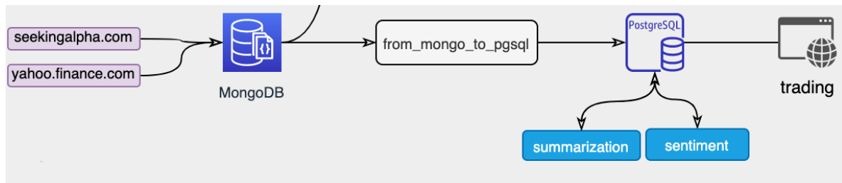
Fig. 5: Illustration of process pipeline
