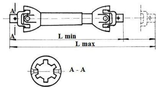
Fig. 15. Propshaft for power transmission from tractor power take-off shaft
