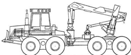
Fig. 96. Prime mover LOKOMO 933 C with the clam bunk
