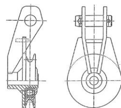
Fig. 80. Open pulley
