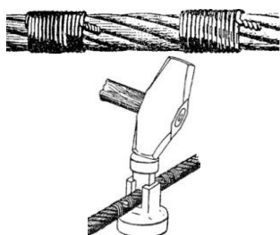
Fig. 58. Cutting cable in the field
