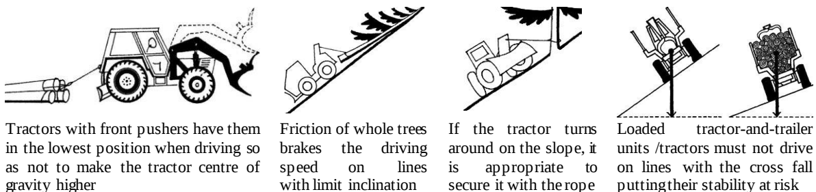
Fig. 118. Some principles of safe timber skidding
