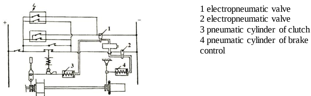
Fig. 67. Schematic of a remote winch control
