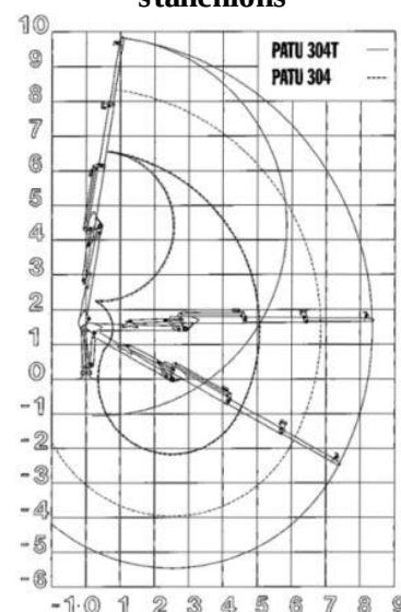
Fig. 107. Diagram of boom reach
