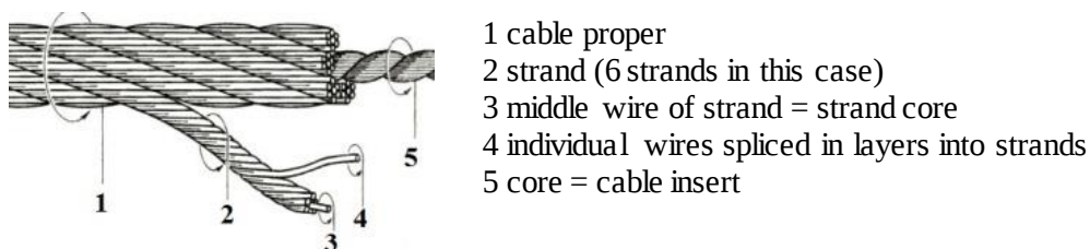
Fig. 49. Cable – Basic parts
