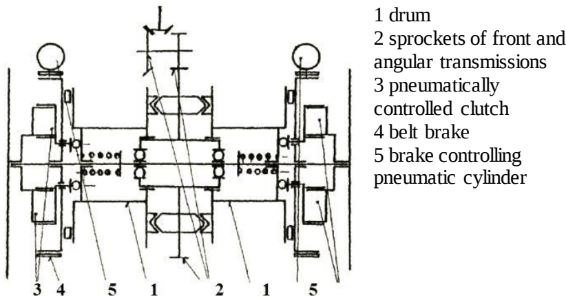
Fig. 70. Schematic of double drum winch
