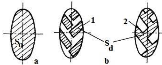
Fig. 33. Tyre bearing surface
