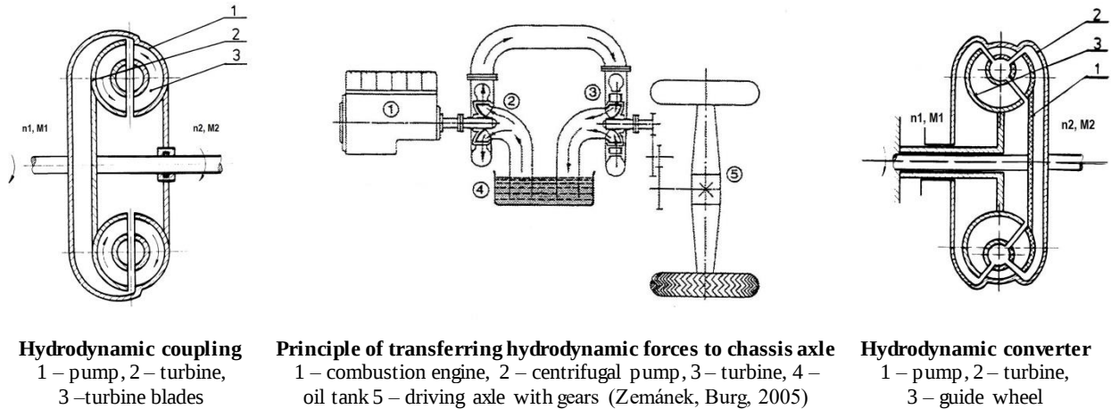
Fig. 47. Hydrodynamic elements and their functions
