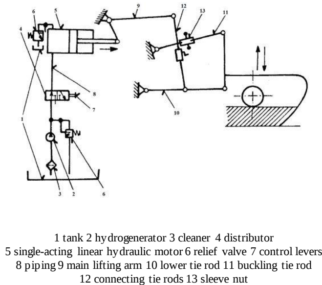
Fig. 16. Hydraulic systems of the tractor
