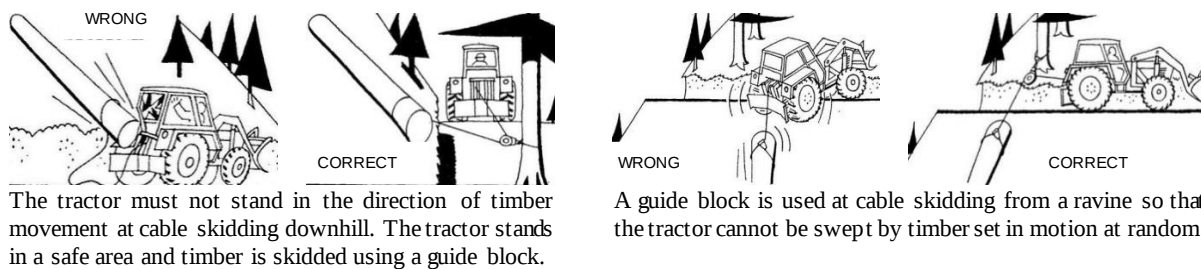
Fig. 117. Winch cable skidding
