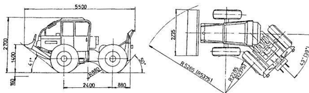
Fig. 23. Forest wheeled prime-mover LKT-81
