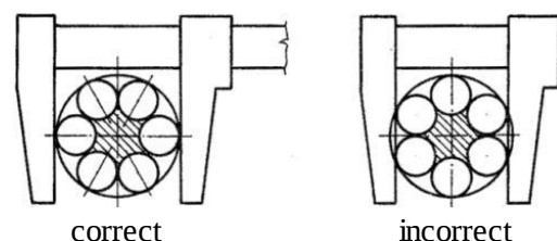
Fig. 52. Measurement of nominal cable diameter
