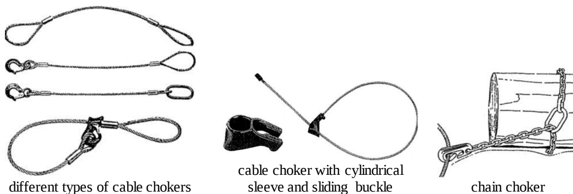
Fig. 63. Chokers
