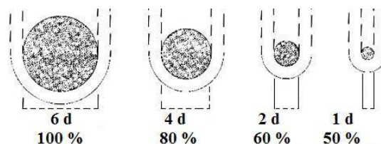
Fig. 85. Cable load carrying capacity in dependence on the inner pulley diameter
