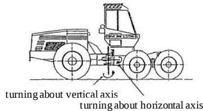
Fig. 7. Central axial joint
