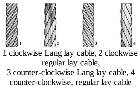
Fig. 51. Cable winding
